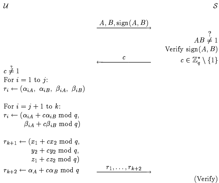
FIGURE 9. Payment protocol for checks
