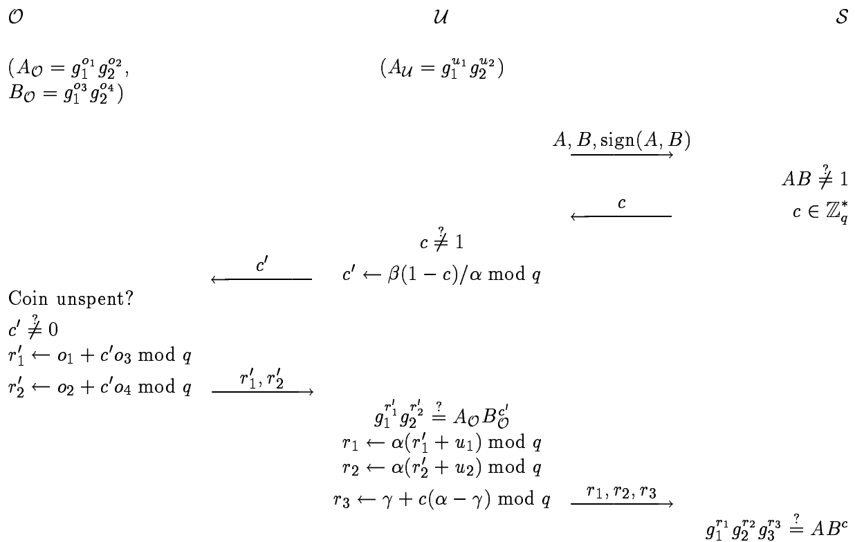
FIGURE 17. The payment protocol for wallets with observers
