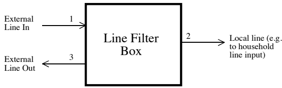
Figure 7. The line filter box (see Figure 1) should be installed at each intersection of the line to separate the non-KLJN communicator loads from the KLJN frequency band [29].
