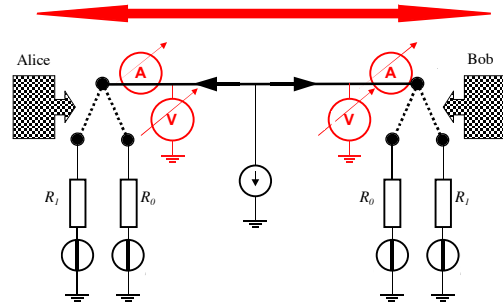
Public channel, broadcasting for comparing instantaneous local current (A) and voltage (V) data
