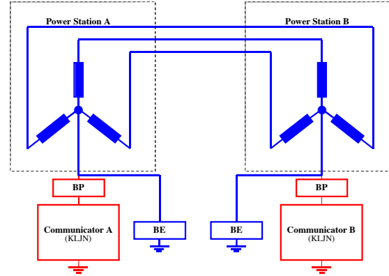
Figure 9. A more robust version [29] of the scheme shown in Figure 8.
