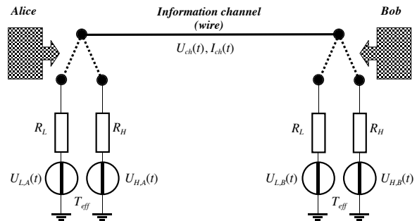
Figure 3. The core of the KLJN secure key exchange system.
