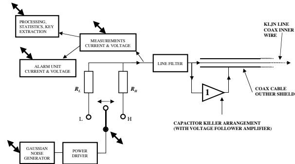
Figure 5. A practical KLJN cypher [18]. Double-headed arrows symbolize computer control.
